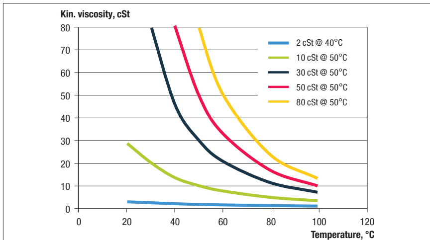
Fig. 5: Temperature – viscosity relationship for low-medium viscosity fuels
